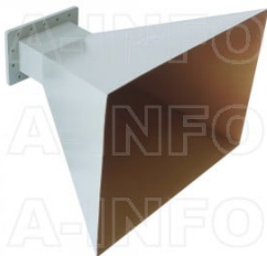
LB-770-15-A Standard Gain Horn Antenna 0.96-1.45GHz 15dB Gain Rectangular Waveguide Interface
