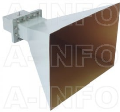
LB-770-15-C-SF Standard Gain Horn Antenna 0.96-1.45GHz 15dB Gain SMA Female
